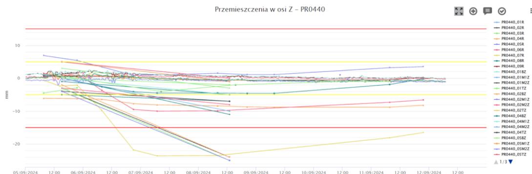
Figure 6-3 Settlement of building PR0440 - Geoscope
