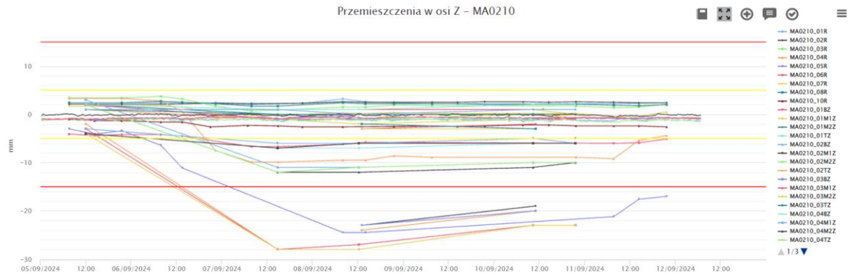
Figure 6-9 Settlement of building MA0210 - Geoscope
