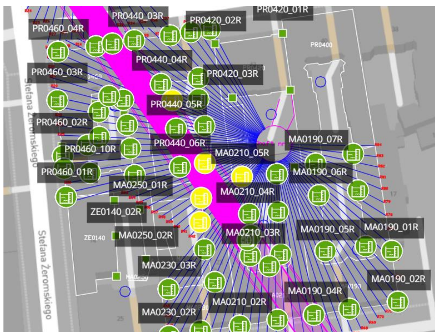
Figure 6-2 Monitoring points – Beyond
